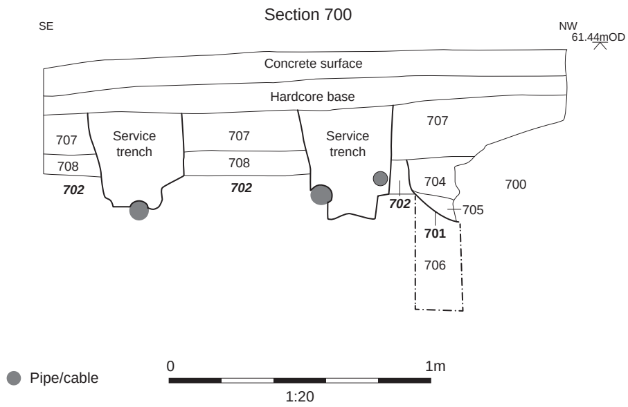
Figure 16: Trench 7, section 700
