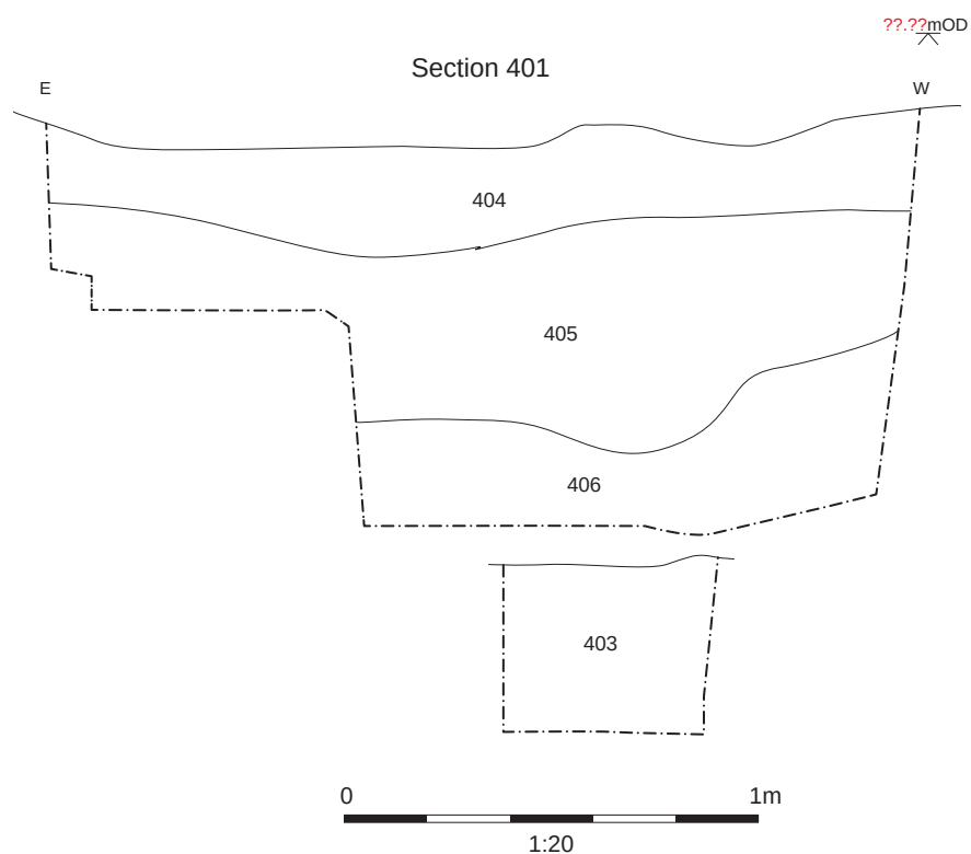
Figure 10: Trench 4, section 401
