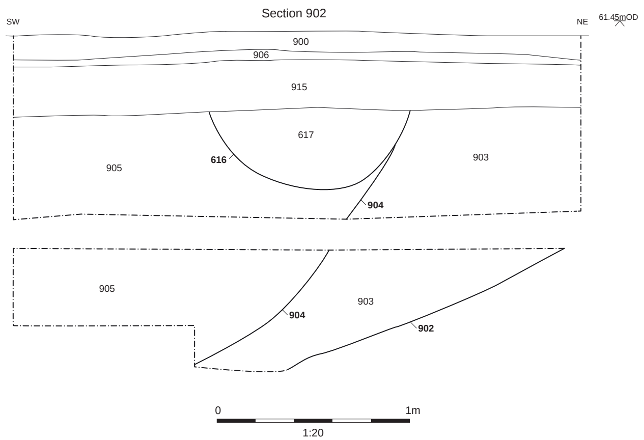
Figure 20: Trench 9, section 902
