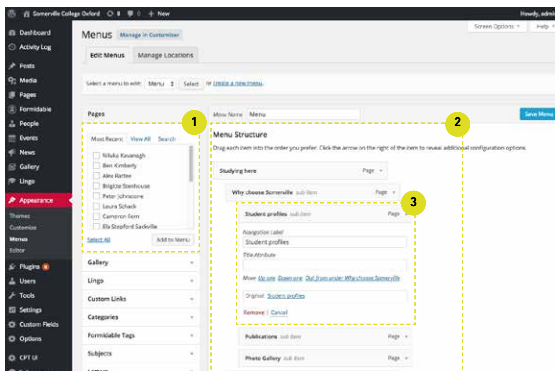
Figure 5.1 Menu page
