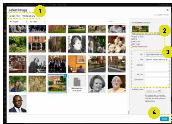
Figure 5.3 Media library
