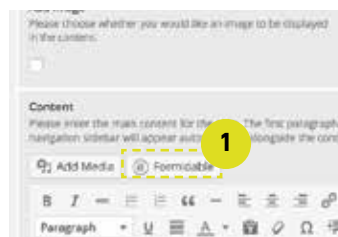
Figure 6.3 Page strip
